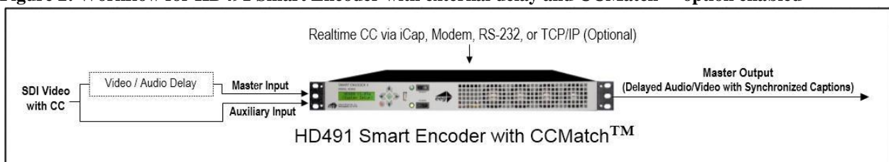
Figure 2: Workflow for HD491 Smart Encoder with external delay and CCMatch™ option enabled
